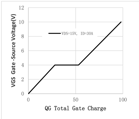
Fig.1 Gate-Charge Characteristics
