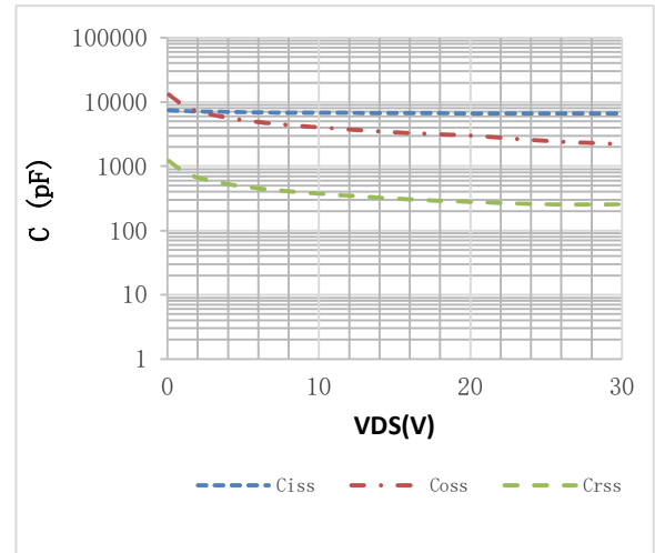
Fig.2 Capacitance Characteristics
