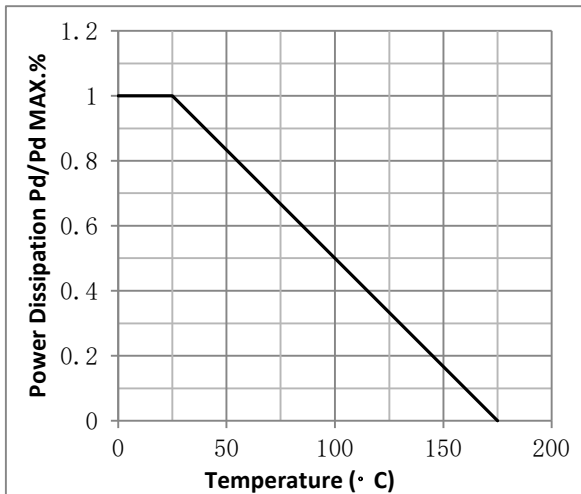
Fig.3 Power Dissipation
